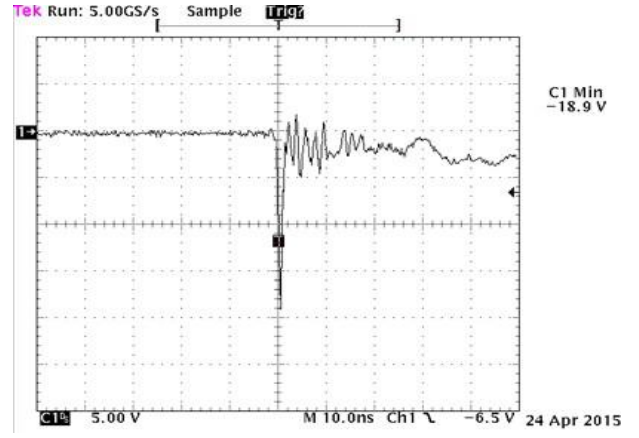
Fig5.Negative 8 kV Contact per IEC61000.4.2
