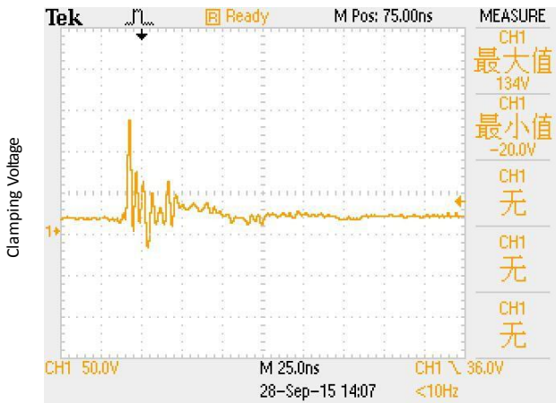
ESD clamping
